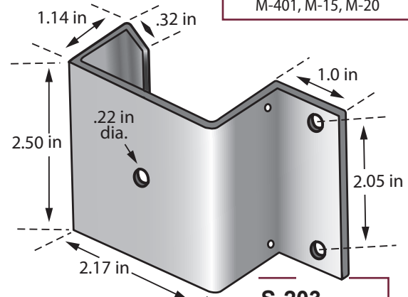
S-203 Garage Door Track Bracket 250, 4400 Series, M-4400, M-250, M-280, M-8, M-14
