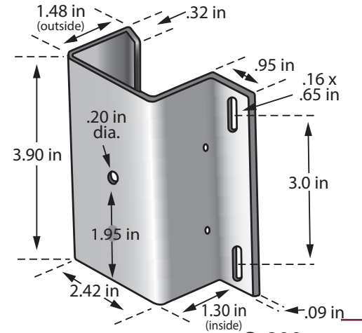
S-200 Garage Door Track Bracket 400 Series M-401, M-15, M-20
